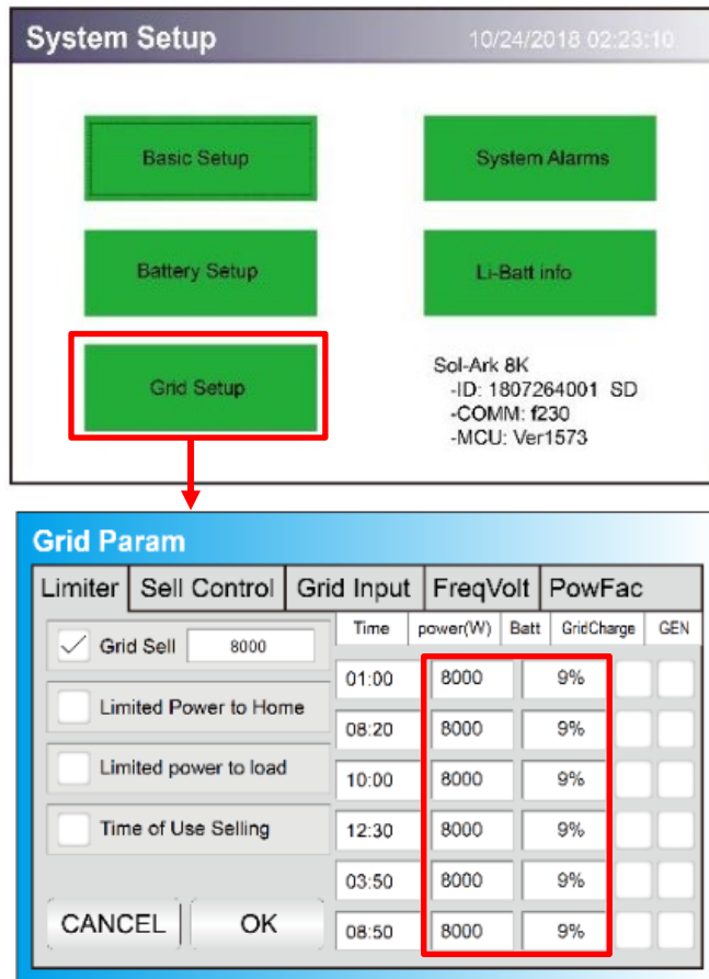
Figure 4 – Limiter Tab in Grid Setup menu
